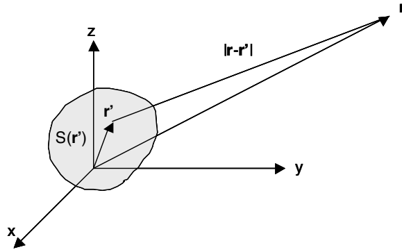
Figure 1. A localized source distribution s(\mathbf{r}') .
