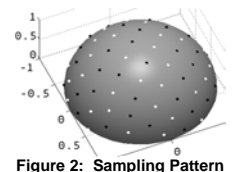
Figure 2: Sampling Pattern
